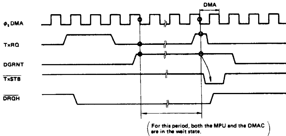
Figure 14 Extraordinary TxRQ Input (1)
