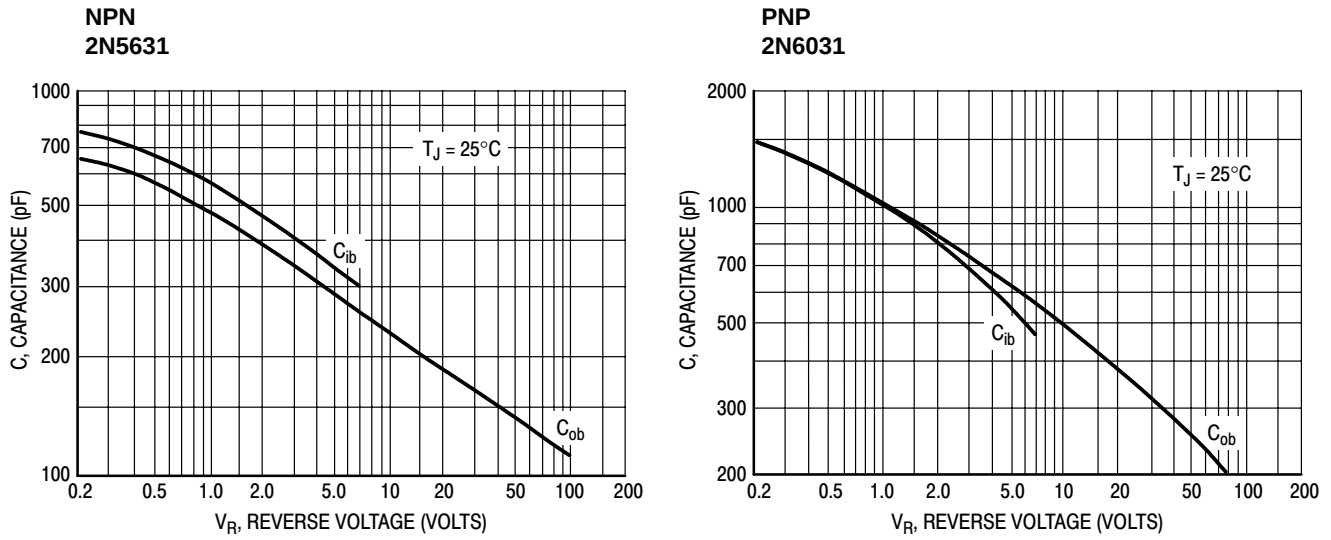
Figure 7. Capacitance
